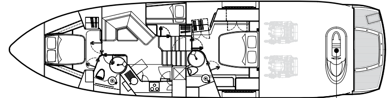
Lower deck with optional crew cabin in lieu of garage
